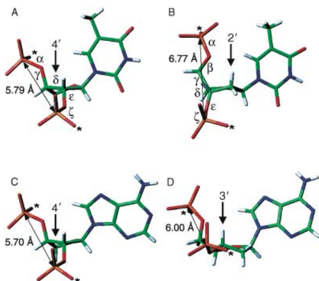
Figure 1. Conformations adopted by TNA and DNA nucleotides in B- and A-form duplexes: a) B-TNA (with residue T*7); b) B-DNA (T20); c) A-TNA (A*7); d) A-DNA (A15). Asterisks in the figure designate the directions of the backbone chain, torsion angles in TNA and DNA are labeled, and carbon atoms of the L- \alpha -threofuranose and D- \beta -deoxyribose sugars positioned either exo (TNA) or endo (DNA) to the best plane (defined by the other sugar ring carbon and oxygen atoms) are indicated by arrows.
