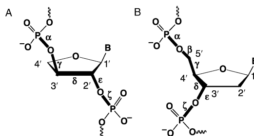
Scheme 1. Configuration, atom numbering, and backbone torsion angle definition in a) TNA and b) DNA.
